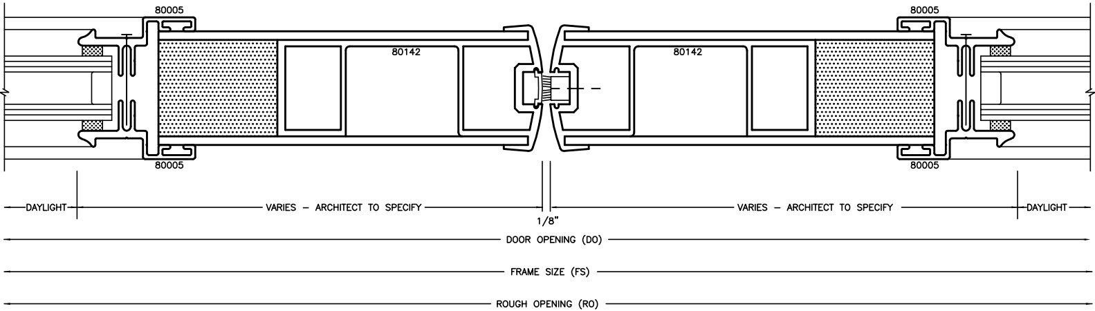
MEETING RAIL - VISION SCALE: (1=1)
