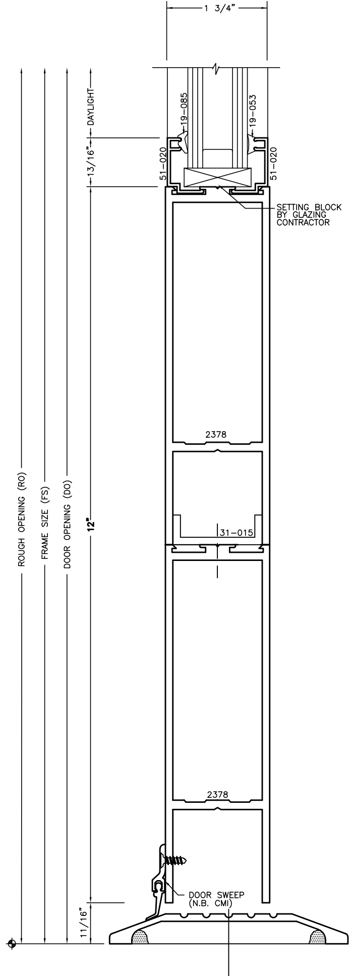
○ 12" STACKED DOOR BOTTOM RAIL SCALE: (1=1)
