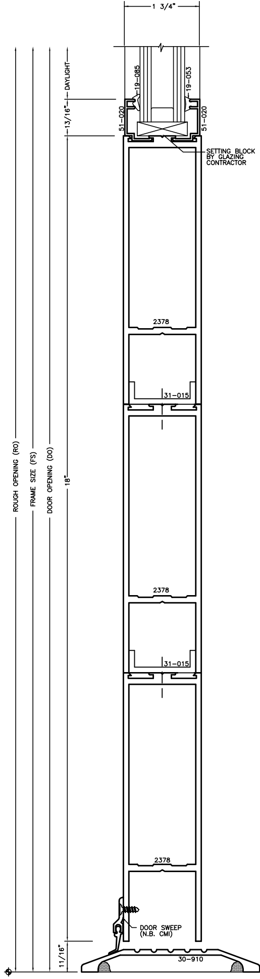
18" STACKED DOOR BOTTOM RAIL SCALE: (1=1)
