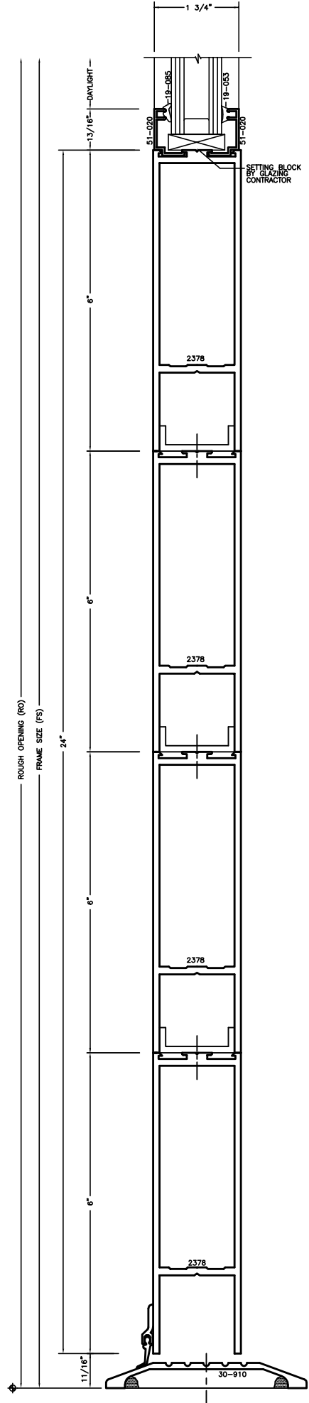
24" 24" STACKED DOOR BOTTOM RAIL SCALE: (1=1)
