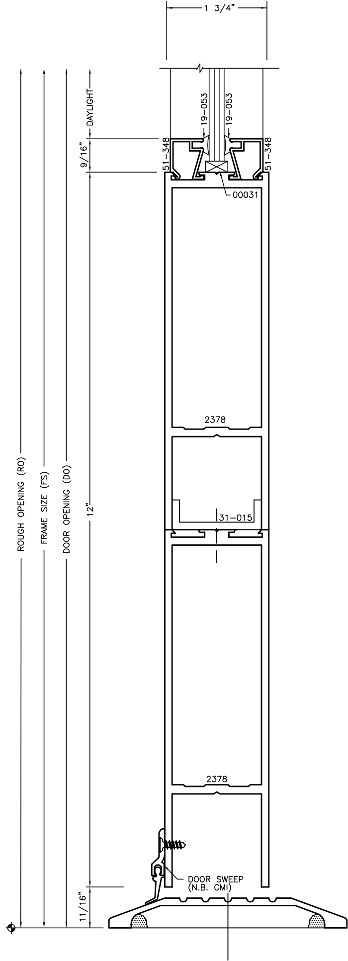
12" STACKED DOOR BOTTOM RAIL SCALE: (1=1)
