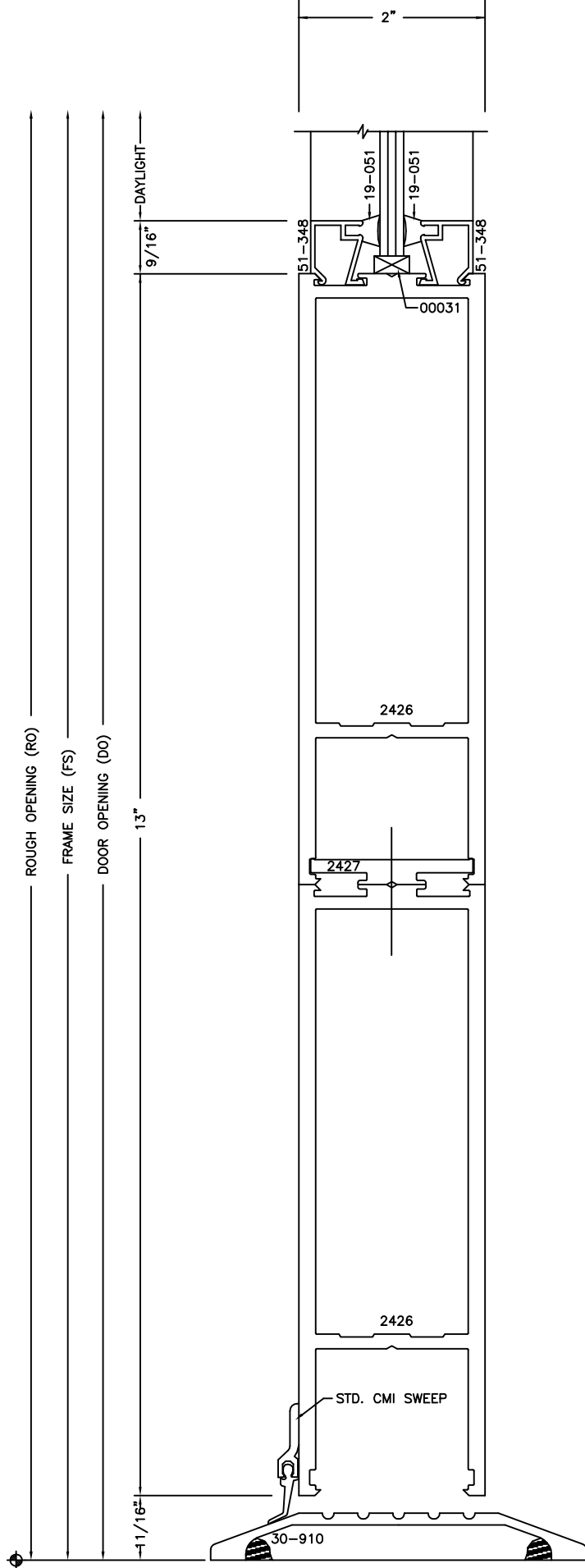
○ 13" HD DOOR BOTTOM RAIL SCALE: (1=1)
